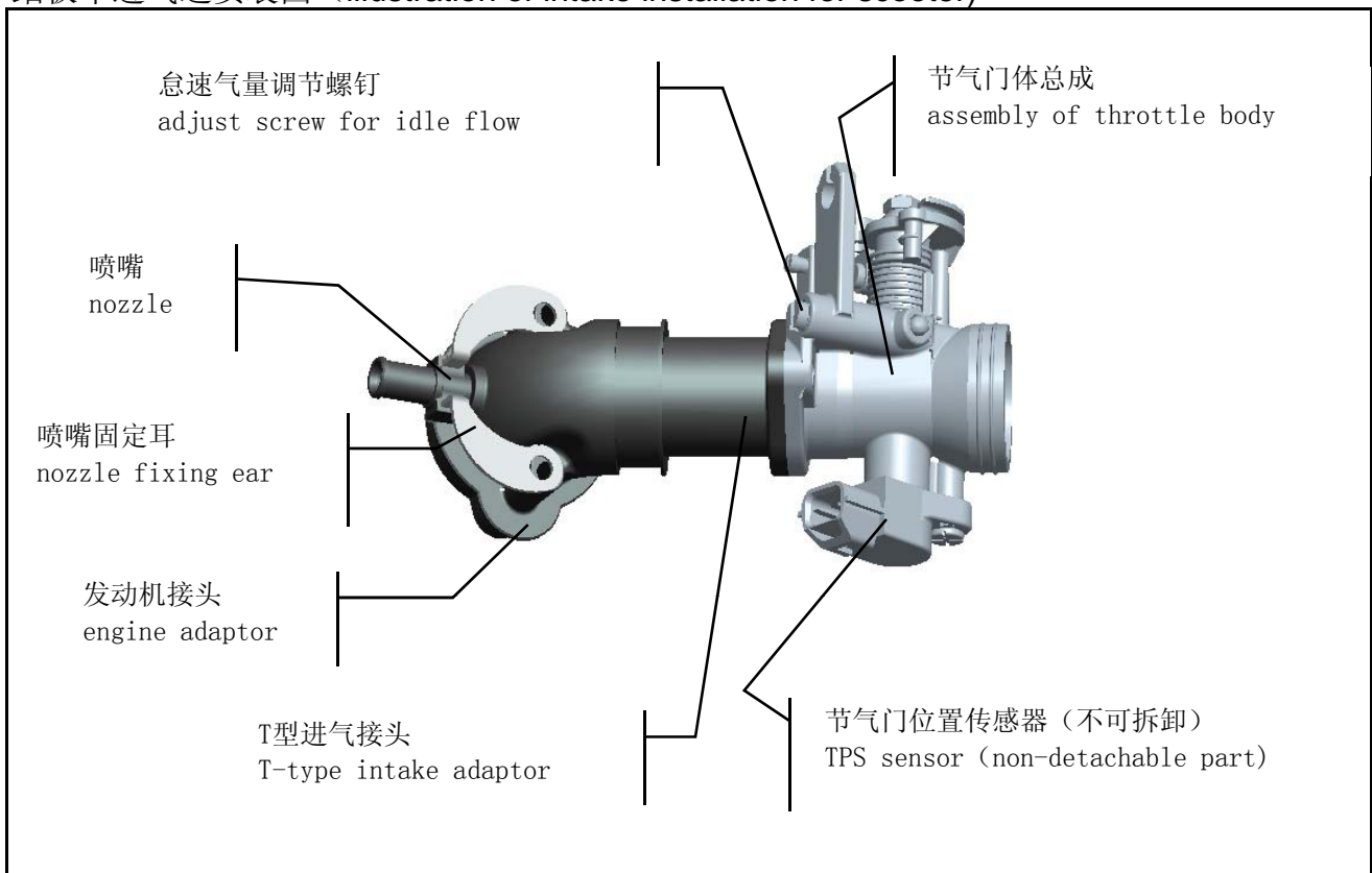
踏板车进气道安装图 (illustration of intake installation for scooter)
